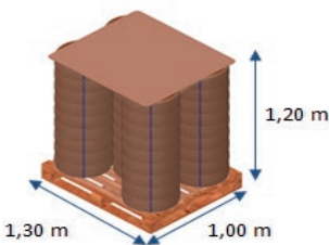
Microirrigation line in coils of 50 m
